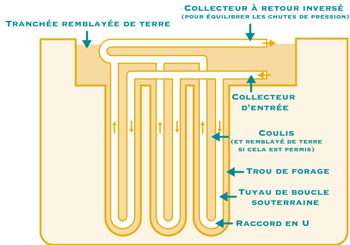
FIGURE 10. BOUCLE SOUTERRAINE VERTICALE
